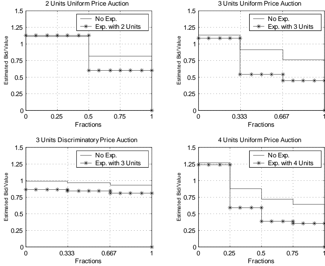
Figure 1: Demand Functions
